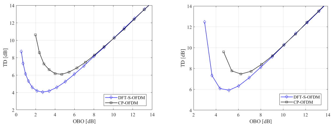
QPSK Modulation (b) 16-QAM modulation Figure 7.3.7.2.1-1: DFT-S-OFDM vs CP-OFDM total degradation
