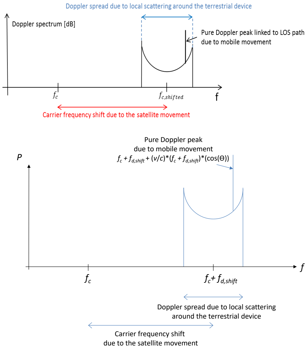
Figure 6.9.2-1: Illustration of Doppler power spectrum in NTN in LOS conditions
